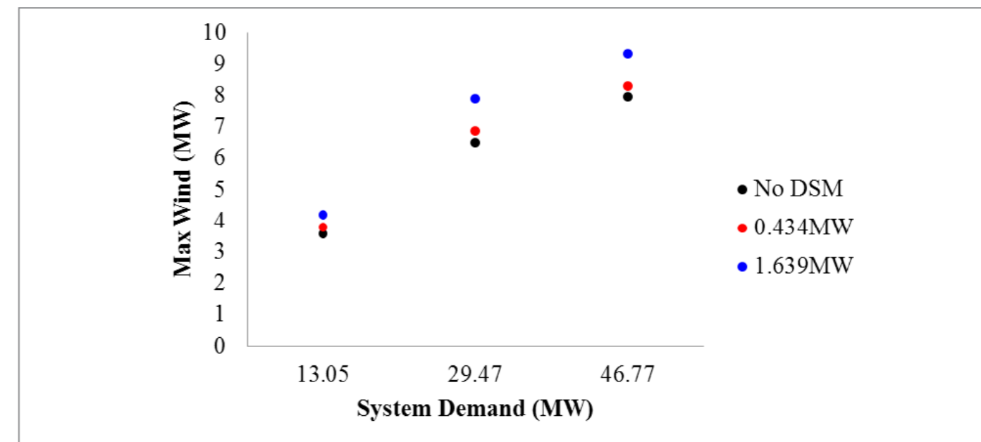
Figure 12: Maximum wind generation (SVT offline)
