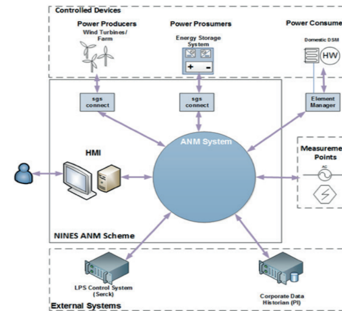
Figure 4: NINES ANM connections
