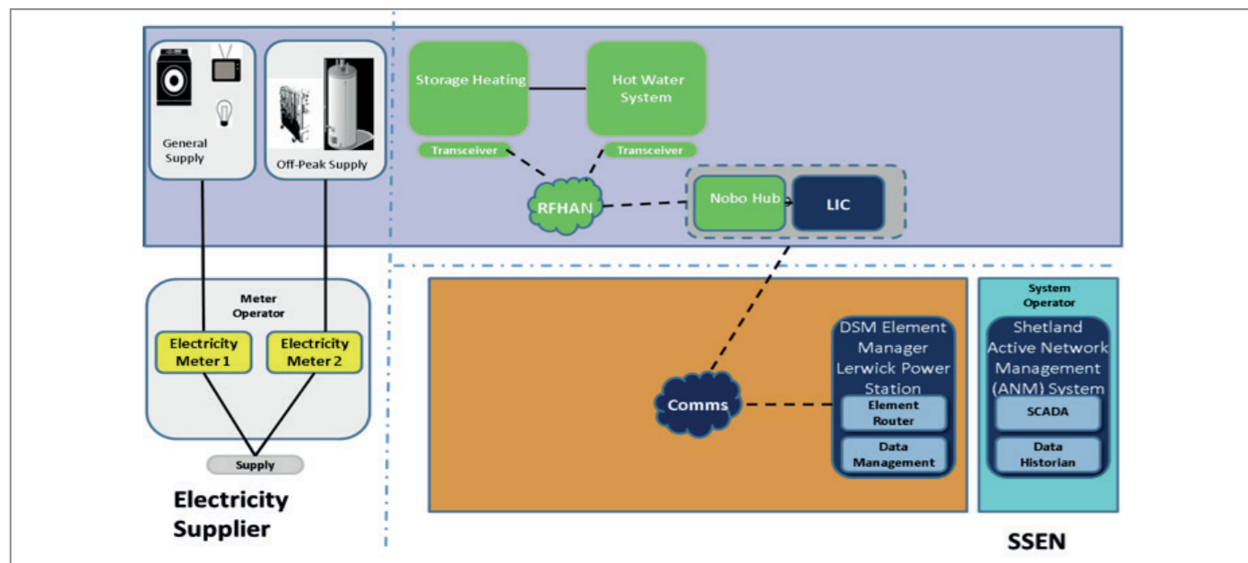
Figure 5: DDSM Infrastructure
