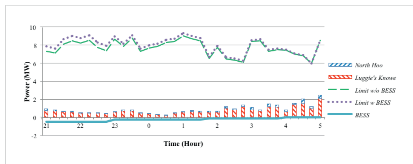
Figure 15 ACG export, Limit w/o BESS and Limit w BESS from 21:00 on 03/11/2016 to 05:00 on 04/11/2016.
