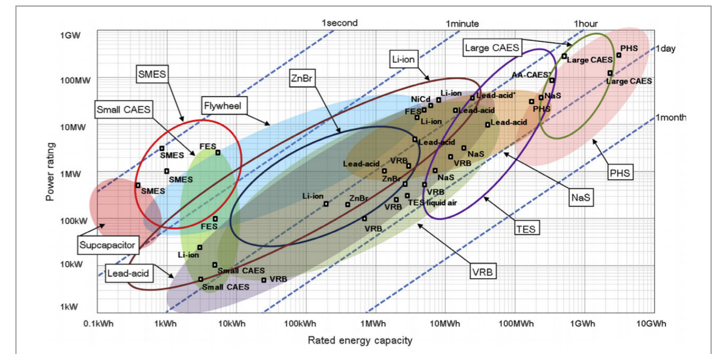
Figure 3 Power ratings and rated energy capacities of different energy storage technologies [3]
