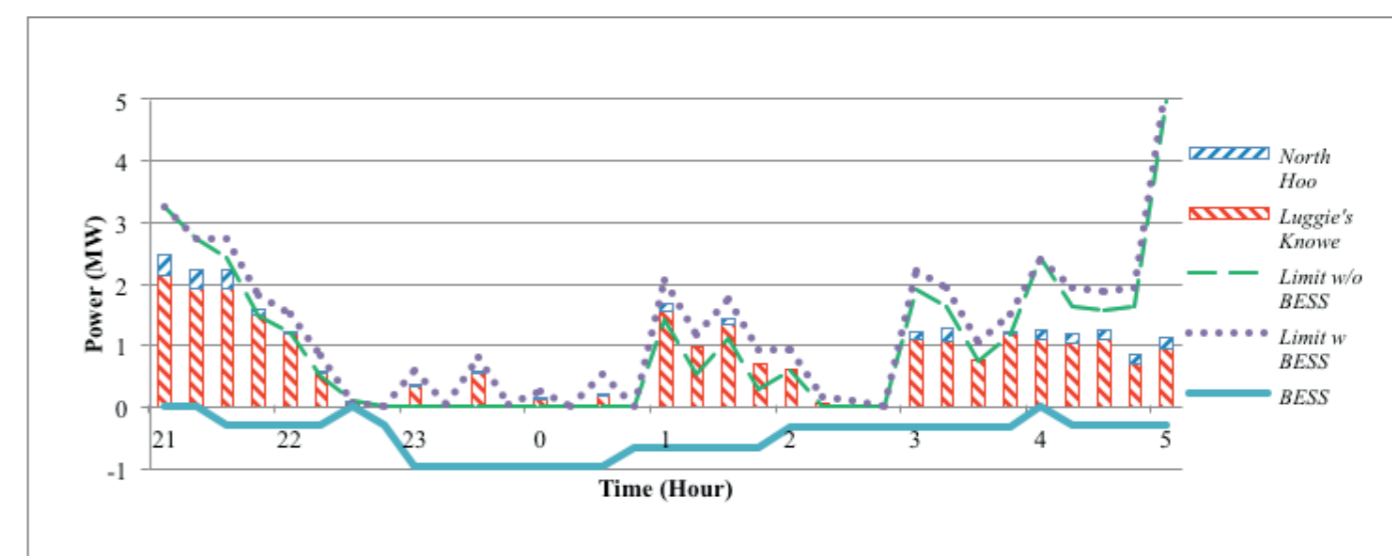
Figure 16 ACG export, Limit w/o BESS and Limit w BESS from 21:00 on 31/03/2016 to 05:00 on 01/04/2016.
